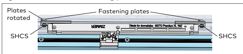
Fig. 20.6 LH DM unit fastening plates secured in track
