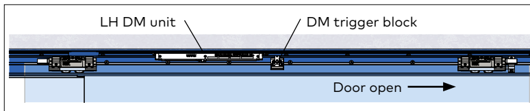
Fig. 20.3 LH DM unit inserted in track
