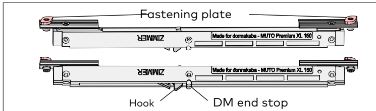
Fig. 20.2 LH DM unit fastening plates rotated
