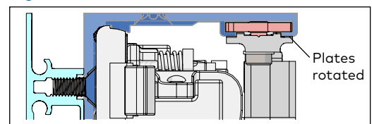
Fig. 20.8 LH DM unit installed in track
