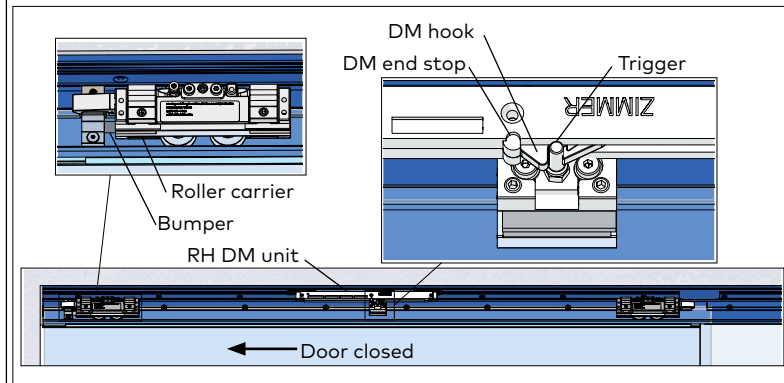
Fig. 19.4 DM unit hook positioned in trigger
