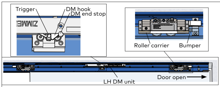
Fig. 20.4 DM unit hook positioned in trigger
