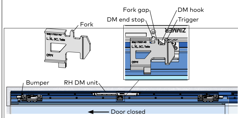
Fig. 19.6 RH DM unit fastening plates secured in track
