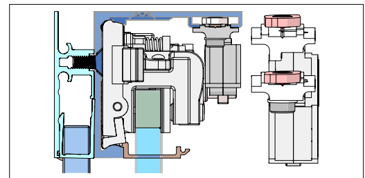
Fig. 20.7 LH DM unit aligned in track
